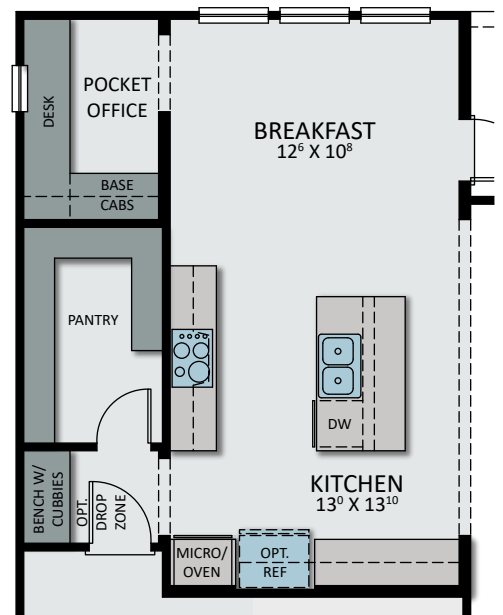
OPT. POCKET OFFICE
